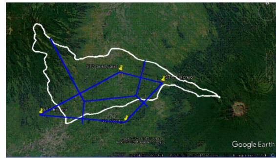
Gambar 4. Polygon Thiessen
