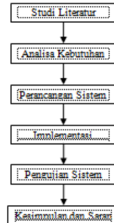
Gambar 1. Alur Penelitian
