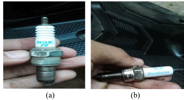
Gambar 2. Busi (a) standar, (b) iridium
