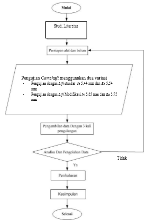
Gambar 1. Metode Penelitian
