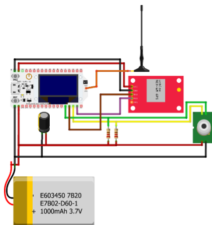
Gambar 2. Schematic STMJ sender
