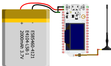
Gambar 4. Schematic STMJ repeater
