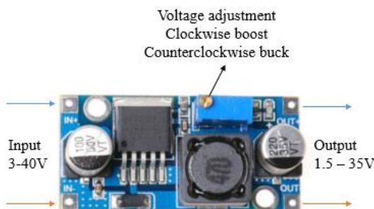
Gambar 3. Regulator LM2596S
