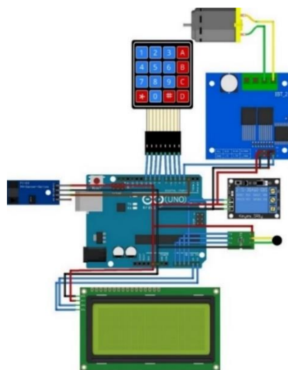
Gambar 3. Wiring Diagram Hot Plate Magnetic Stirrer Berbasis Arduino Uno
