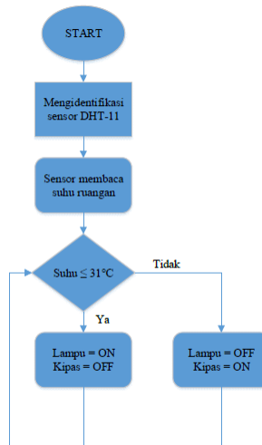
Gambar 5. Flowchart sistem kontrol suhu otomatis
