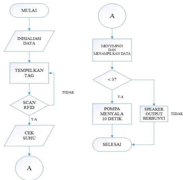
Gambar 3. Flowchart
