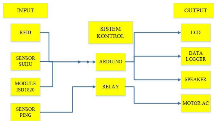
Gambar 1. Blok diagram
